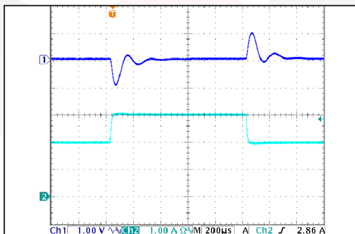
Figure 11: Output voltage response to step-change in load current (50%-75%-50% of I_{out(max)} ; dI/dt = 0.1 \text{ A}/\mu\text{s} ). Load cap: 1 μF ceramic and 15 μF tantalum capacitors. Ch 1: V_{out} (1V/div), Ch 2: I_{out} (1A/div).
