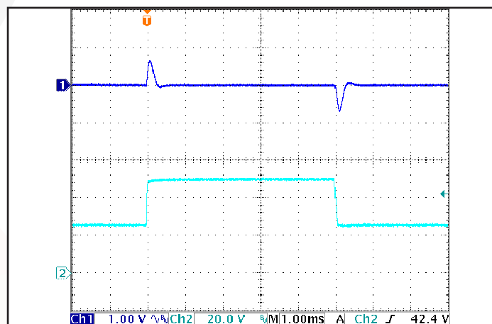
Figure 12: Output voltage response to step-change in input voltage (250V/ms). Load cap: 100 μF electrolytic output capacitance. Ch 1: V_{out} (1V/div), Ch 2: V_{in} (20V/div).
