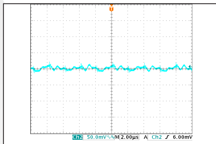
Figure 10: Output voltage ripple, V_{out} , at nominal input voltage and rated load current (50 mV/div). Load capacitance: 1μF ceramic capacitor and 15μF tantalum capacitor. Bandwidth: 10 MHz. See Figure 17.
