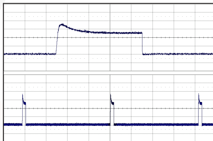
Figure 18: Load current (2A/div) as a function of time (2ms/div and 50ms/div) when the converter attempts to turn on into a 10 mΩ short circuit.
